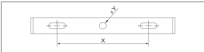
Fig.10: Wall mounting
