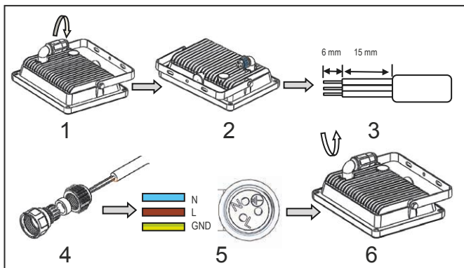
Fig.5: Installation
